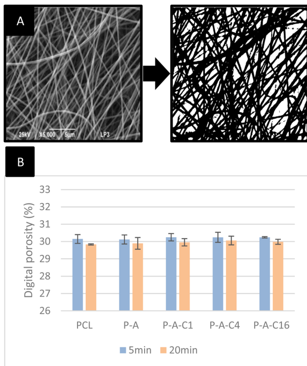
Fig. 4 Digital evaluation of the porosity of electrospun nanofibers. (A) Example of 70% thresholding on a P-A-C4 sample micrograph. (B) Digital porosity of the membranes electrospun over 5 or 20 minutes. Asterisks on bars represent a statistically significant variation in porosity when compared to the 5 minutes electrospinning duration (one-factor ANOVA followed by Tukey HSD, p < 0.05 ).
